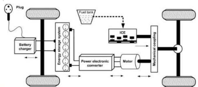
Figure 1 Hybrid electric vehicle block diagram [3]
